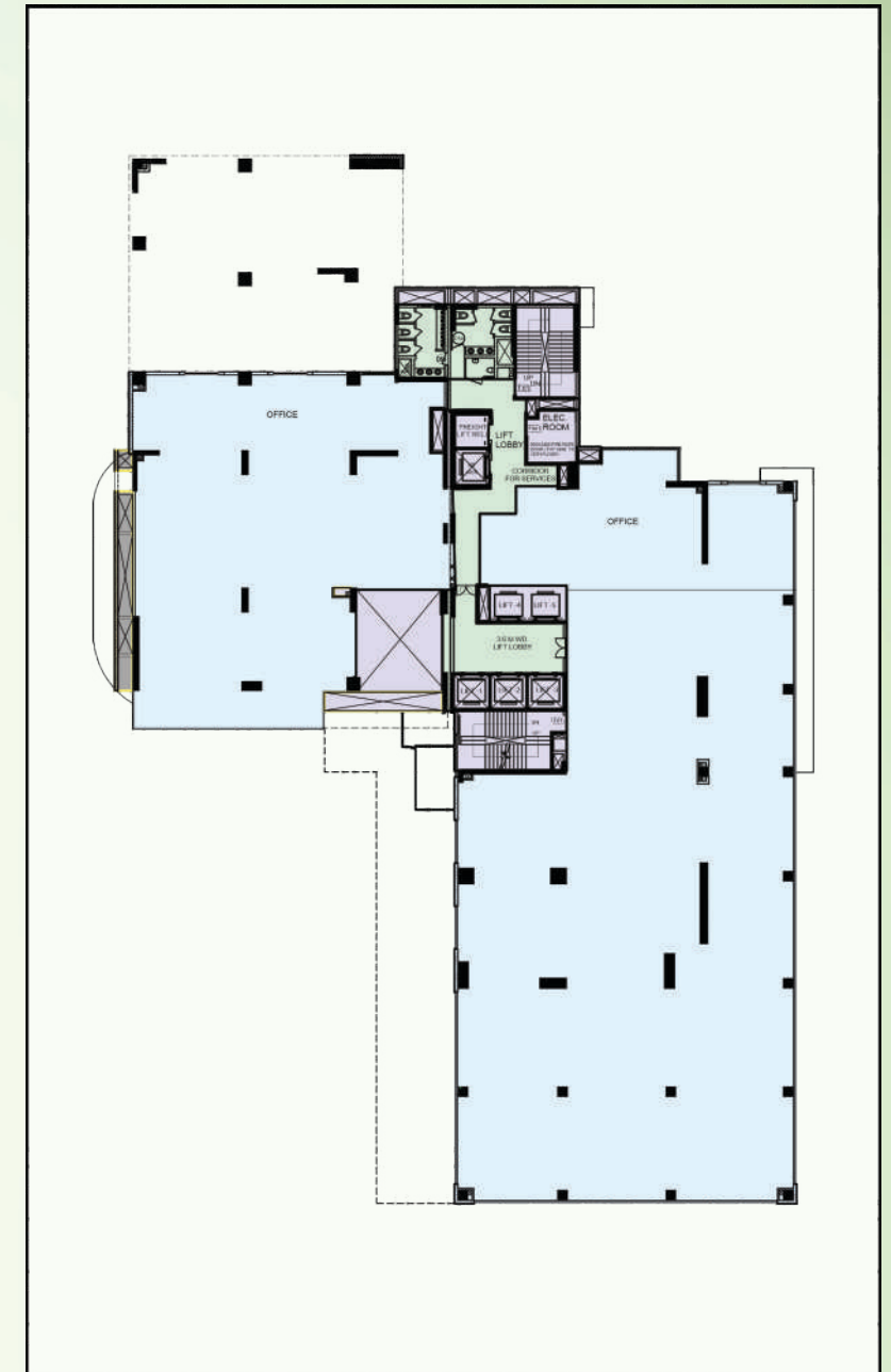
FIRST FLOOR
